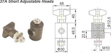
N237A Short Adjustable Heads
