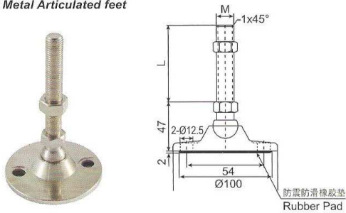
MD100 Metal Articulated feet
