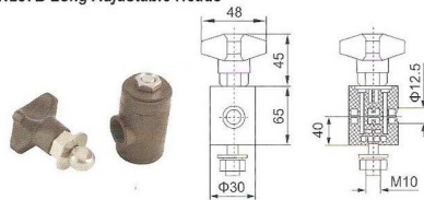
N237B Long Adjustable Heads
