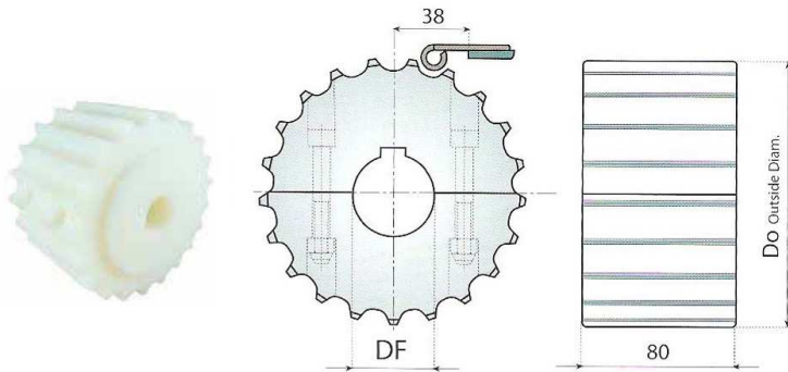
SPLIT SPROCKETS (MACHINED)
