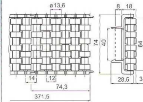
N316-4 Quadruplicate Roller Side Guide (Sideflexing)
