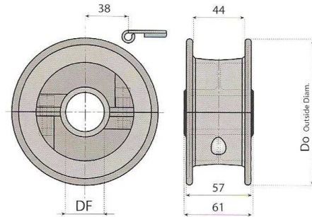
SPLIT IDLER WHEELS ( INJECTION )
