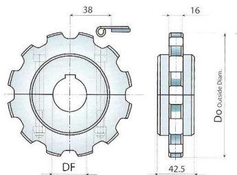
SPLIT SPROCKETS ( MACHINED )
