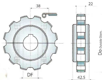
SPLIT SPROCKETS ( MACHINED )
