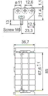
N302 Modular Transfer Roller Plates
