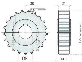
SPLIT SPROCKETS ( MACHINED )
