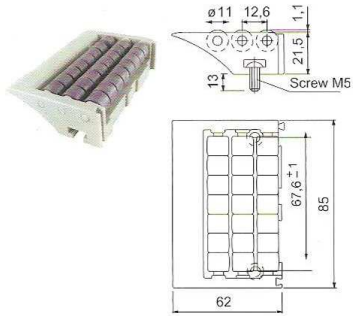
N301 Modular Transfer Roller Plates
