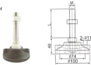
FD100 Fixed feet
