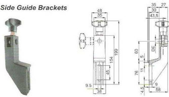
N240 Side Guide Brackets
