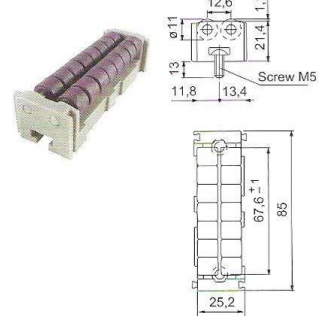
N303 Modular Transfer Roller Plates
