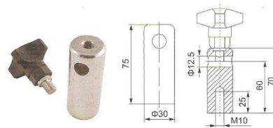
N237D Copper Adjustable Heads
