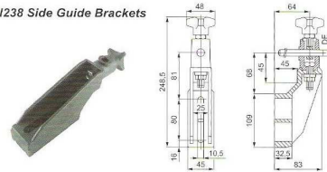
N238 Side Guide Brackets
